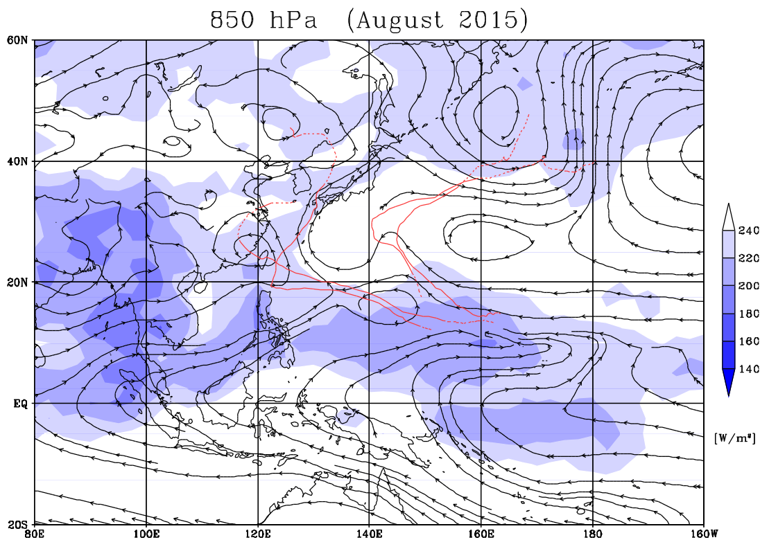
Figure 3.1 Monthly mean streamlines at 850 hPa (lines with arrows) and areas with OLR values of less than 240 W/m^2 (shaded) for August 2015. The tracks of the four named TCs that formed in August are superimposed onto the figure.
